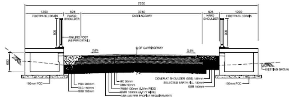
TYPE 2B - TYPICAL PAVEMENT CROSS SECTION - RAISING WITH GSB / CUTTING (DRAIN BOTH SIDES)
